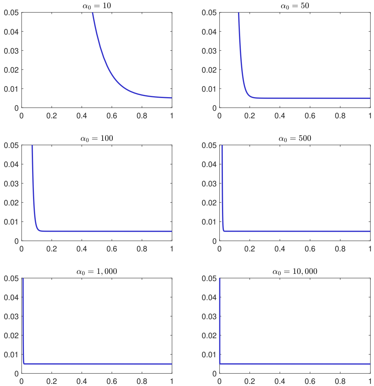
Figure 1: Spike-and-slab Priors for \sigma_i^2
